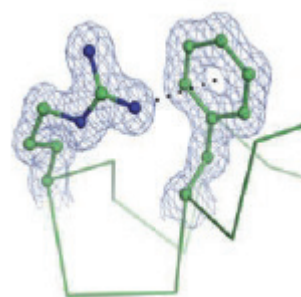
Figure 2. N-H... \pi interaction between the only Arg and Phe68 ( 2F_o - F_c electron density map contoured at 1.2\sigma ).
